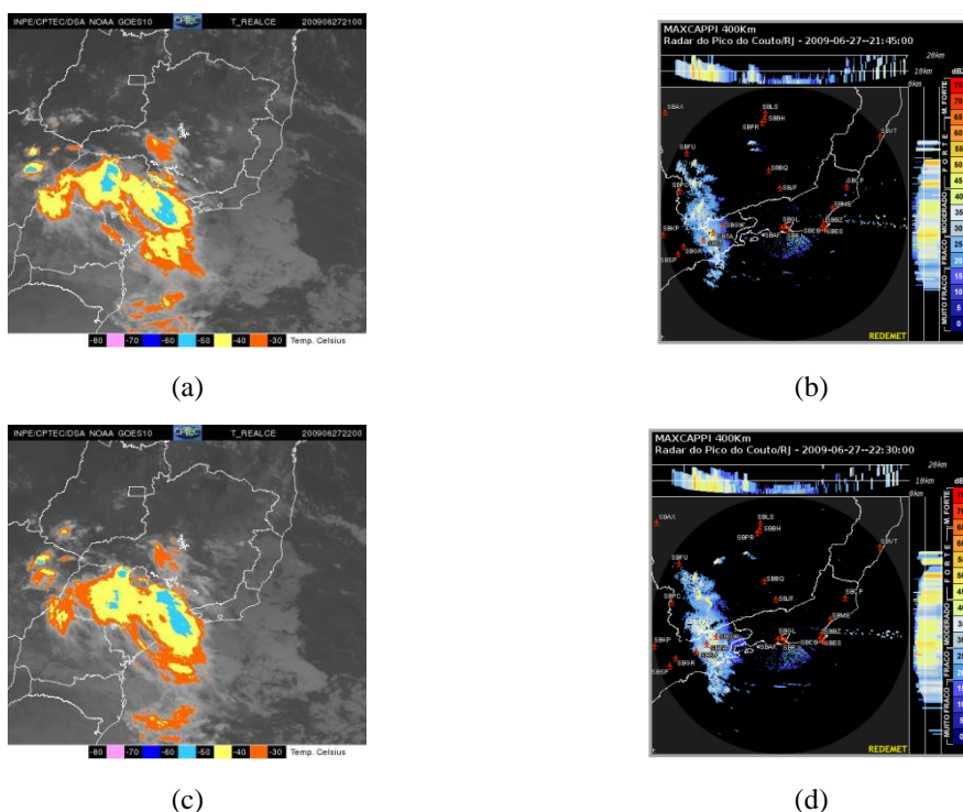
Figure 4: Enhanced and sectorized images of the GOES-10 satellite and images of the Pico de Couto radar on June 27, 2009, (a) at 21:00Z, (b) at 21:45Z, (c) at 22:00Z and (d) at 22:30Z. (Source: CPETC and REDEMET)
