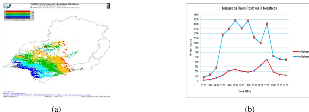
Figure 3: (a) Distribution of lightning flashes throughout the Southeast region, color coded in time. (b) Rate per hour of lightning for the same region. (Source: ELAT/INPE)
