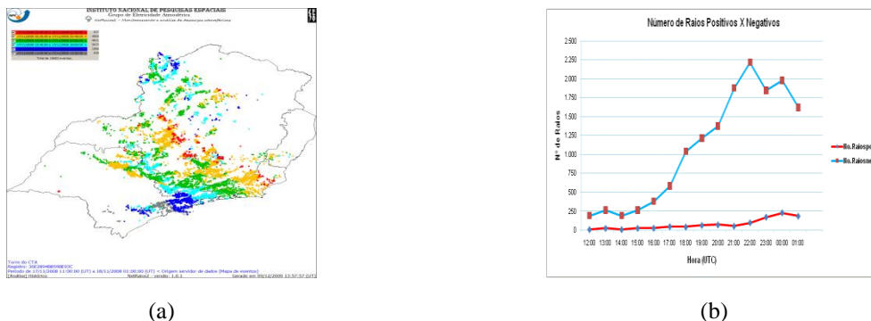
Figure 1: (a) Distribution of lightning flashes throughout the Southeast region, color coded in time. (b) Rate per hour of lightning for the same region. (Source: ELAT/INPE)
